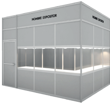
Example modular CLOSED PACK (4x3) + 6 glass show case + 1 door
